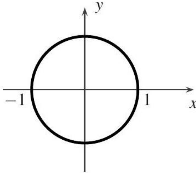
Fig. B.1. The unit circle.
