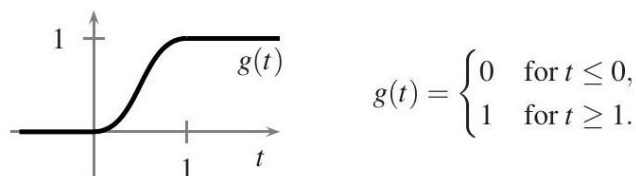
Fig. 13.4. The graph of g(t) .
