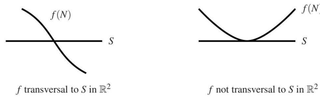
Fig. 9.5. Transversality.
