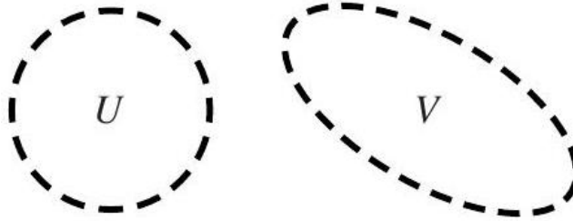
Fig. A.10. A disconnected space.
