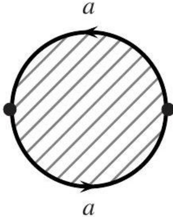
Fig. 28.9. The real projective plane.
