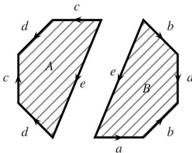
Fig. 28.8. Two halves of a surface of genus 2 .
