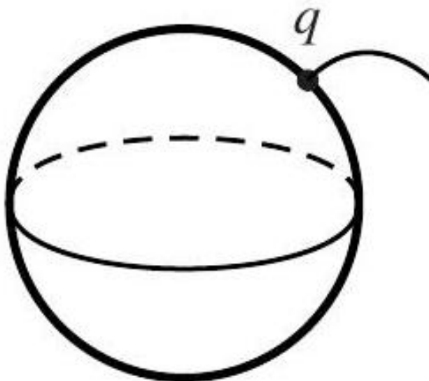
Fig. 5.10. A sphere with a hair.
