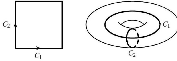
Fig. 28.2. Two closed curves on a torus.
