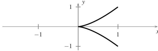
Fig. 8.2. A cuspidal cubic.
