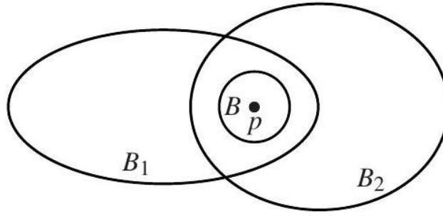
Fig. A.3. Criterion for a basis.
