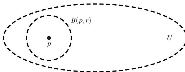
Fig. A.1. An open set in \mathbb{R}^n .
