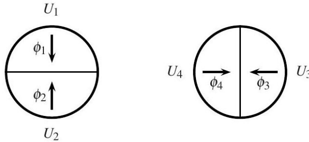
Fig. 5.7. Charts on the unit circle.
