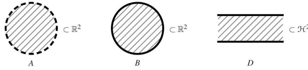
Fig. 22.4. Interiors and boundaries.
