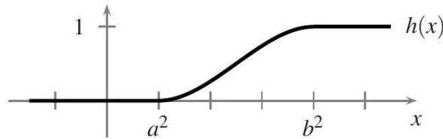
Fig. 13.5. The graph of h(x) .
