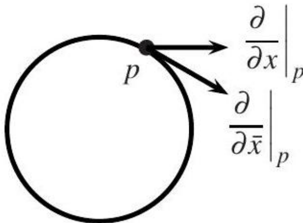
Fig. 11.9. Tangent vector \frac{\partial}{\partial \bar{x}} \Big|_p to a circle.
