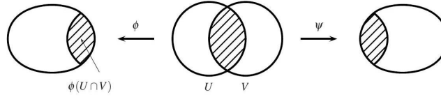
Fig. 5.2. The transition function \psi \circ \phi^{-1} : \phi(U \cap V) \rightarrow \psi(U \cap V) is defined on \phi(U \cap V) .
