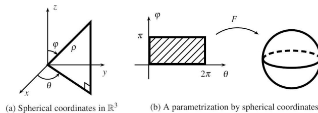
Fig. 23.3. The sphere as a parametrized set.
