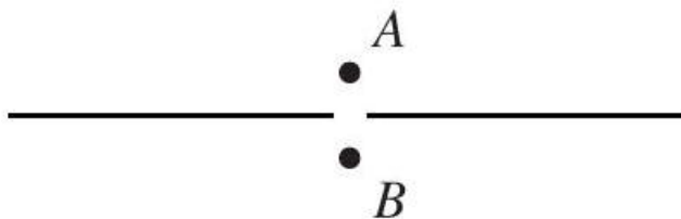
Fig. 5.9. Real line with two origins.
