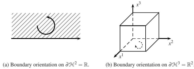
Fig. 22.6. Boundary orientations.
