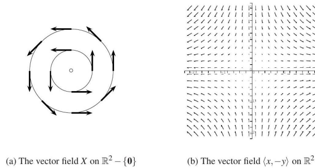
Fig. 2.3. Vector fields on open subsets of \mathbb{R}^2 .
