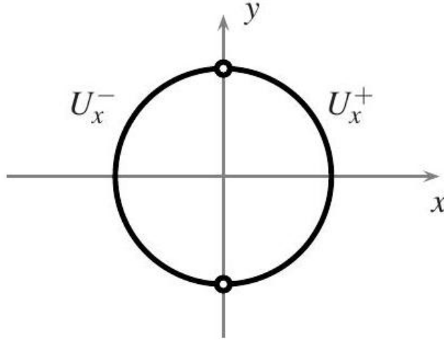
Fig. 19.2. Two charts on the unit circle.
