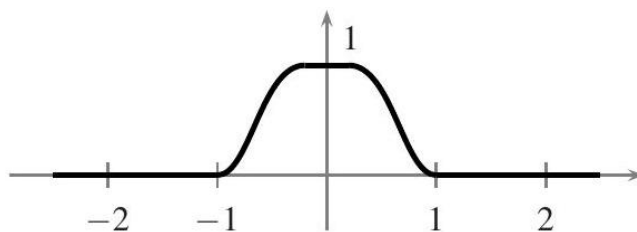
Fig. 13.1. A bump function at 0 on \mathbb{R} .
