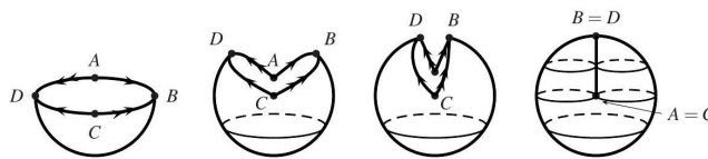
Fig. 7.8. The real projective plane immersed as a cross-cap in \mathbb{R}^3 .
