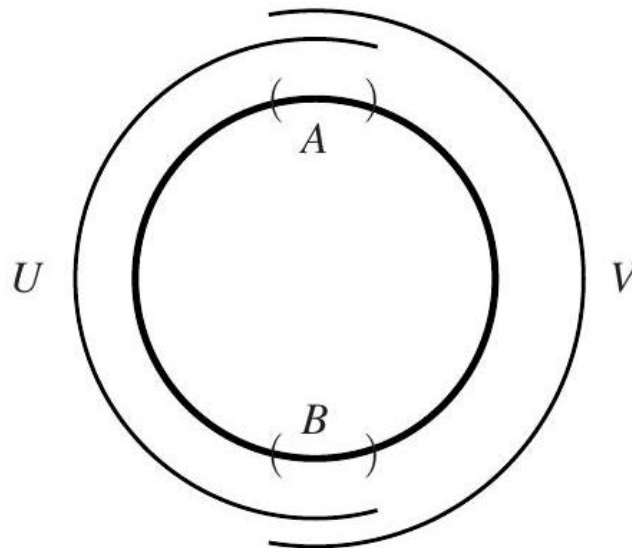
Fig. 26.2. An open cover of the circle.
