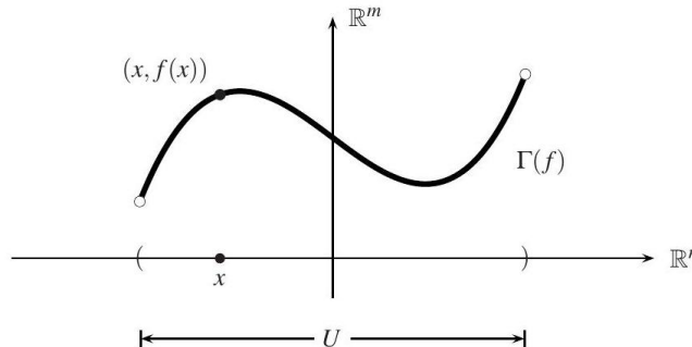
Fig. 5.6. The graph of a smooth function f : U \rightarrow \mathbb{R}^m where U \subset \mathbb{R}^n .
