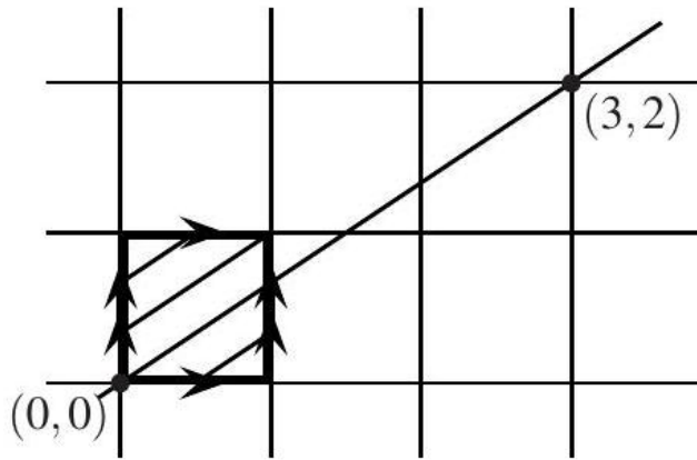
Fig. 15.1. An embedded Lie subgroup of the torus.
