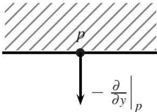
Fig. 22.5. A tangent vector at the boundary.
