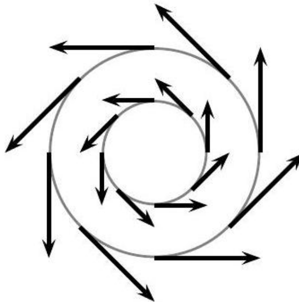
Fig. 12.4. The vector field (-y, x) in \mathbb{R}^2 .
