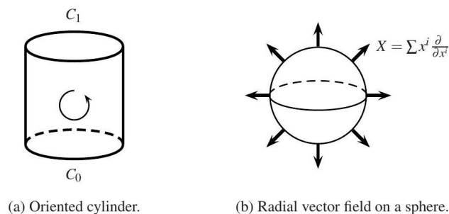
Fig. 22.7. Boundary orientations.
