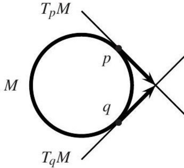
Fig. 12.1. Tangent spaces to a circle.
