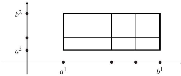
Fig. 23.1. A partition of a closed rectangle.
