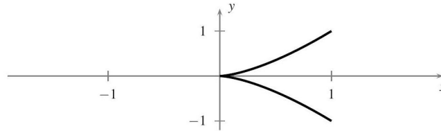
Fig. 11.2. A cuspidal cubic, not an immersion.
