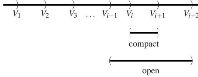
Fig. C.1. A nested open cover.
