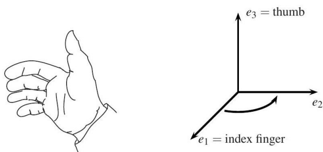
Fig. 21.3. Right-handed orientation (e_1, e_2, e_3) of \mathbb{R}^3 .
