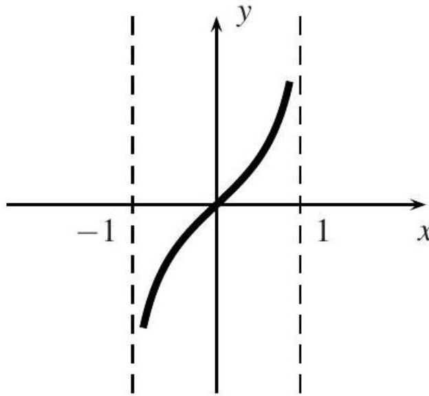
Fig. 23.2. The function f(x) = \tan(\pi x/2) on ] -1, 1[ .
