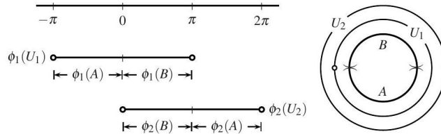
Fig. 5.3. A C^\infty atlas on a circle.
