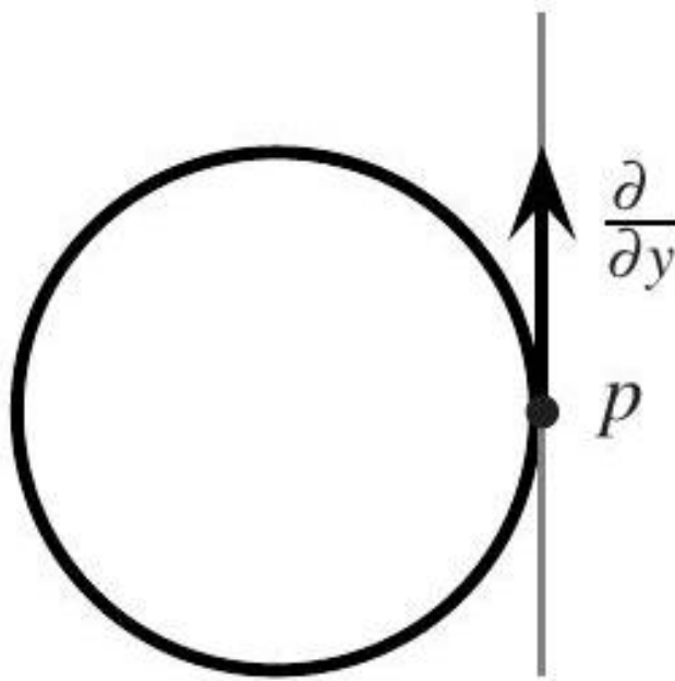
Fig. 19.1. The tangent space to S^1 at p = (1, 0) .
