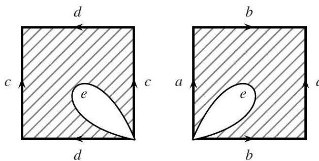
Fig. 28.7. Two halves of a surface of genus 2 .
