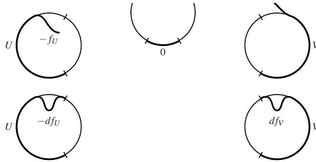
Fig. 26.3. A generator of H^1(S^1) of the circle.
