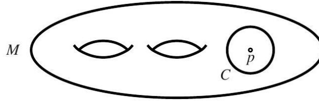
Fig. 28.3. Punctured surface.
