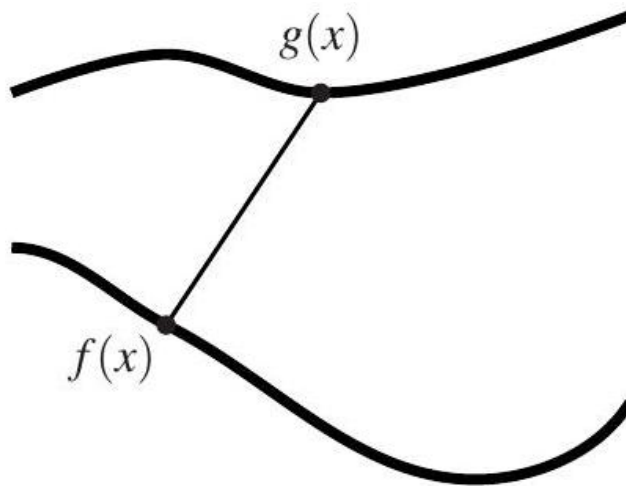
Fig. 27.1. Straight-line homotopies.
