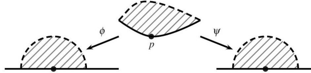
Fig. 22.3. Boundary charts.
