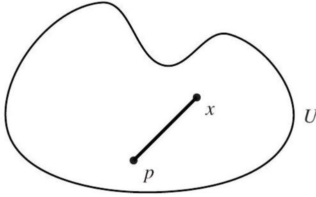
Fig. 1.3. The line segment from p to x .
