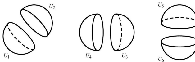
Fig. 5.11. Charts on the unit sphere.
