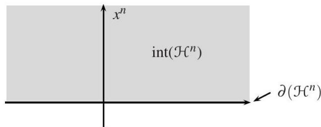
Fig. 22.1. Upper half-space.
