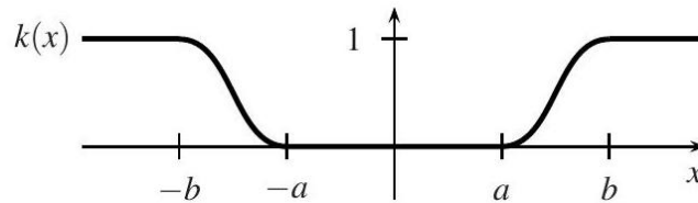
Fig. 13.6. The graph of k(x) .
