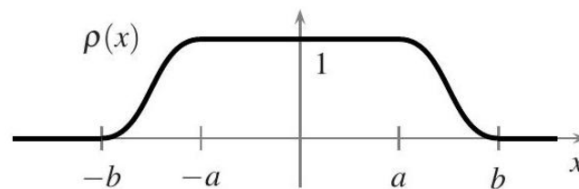
Fig. 13.7. A bump function at 0 on \mathbb{R} .
