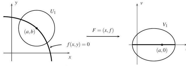
Fig. B.2. F^{-1} F maps the u -axis to the zero set of f .
