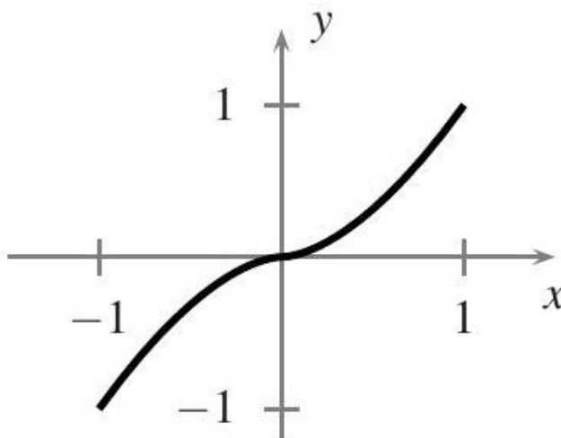
Fig. 13.2. The graph of y = x^{5/3} .
