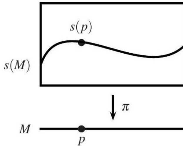
Fig. 12.3. A section of a vector bundle.
