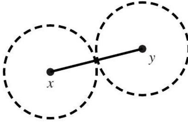
Fig. A.6. Two disjoint neighborhoods in \mathbb{R}^n .
