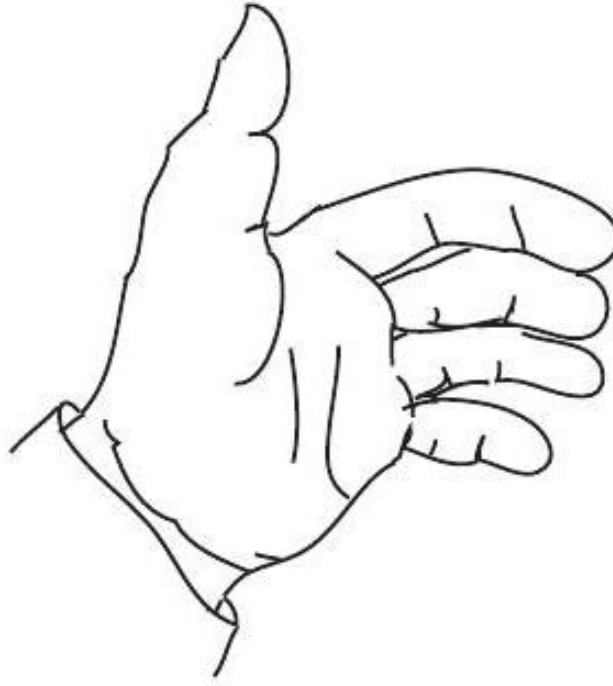
Fig. 21.4. Left-handed orientation (e_2, e_1, e_3) of \mathbb{R}^3 .
