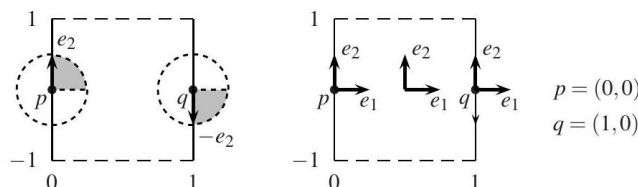
Fig. 21.6. Nonorientability of the Möbius band.
