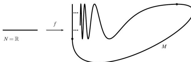
Fig. 11.5. A one-to-one immersion that is not an embedding.
