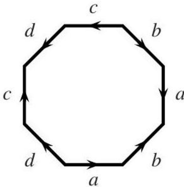
Fig. 28.5. A surface of genus 2 as a quotient space of an octagon.
